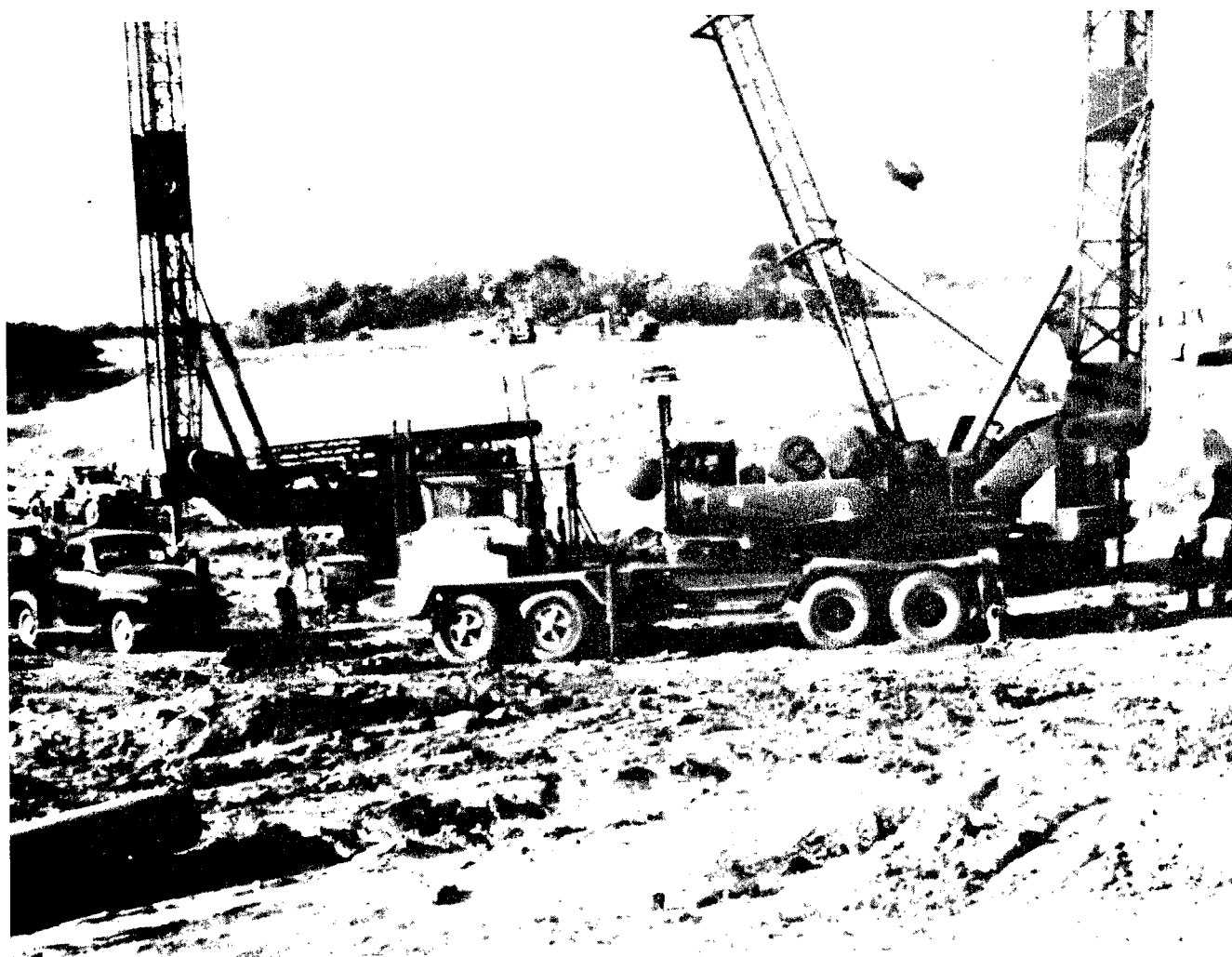
Fig. 3. View of flight auger drill rigs. Photo-USCE.
